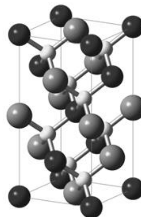
Fig. 1 Chalcopyrite structure.
